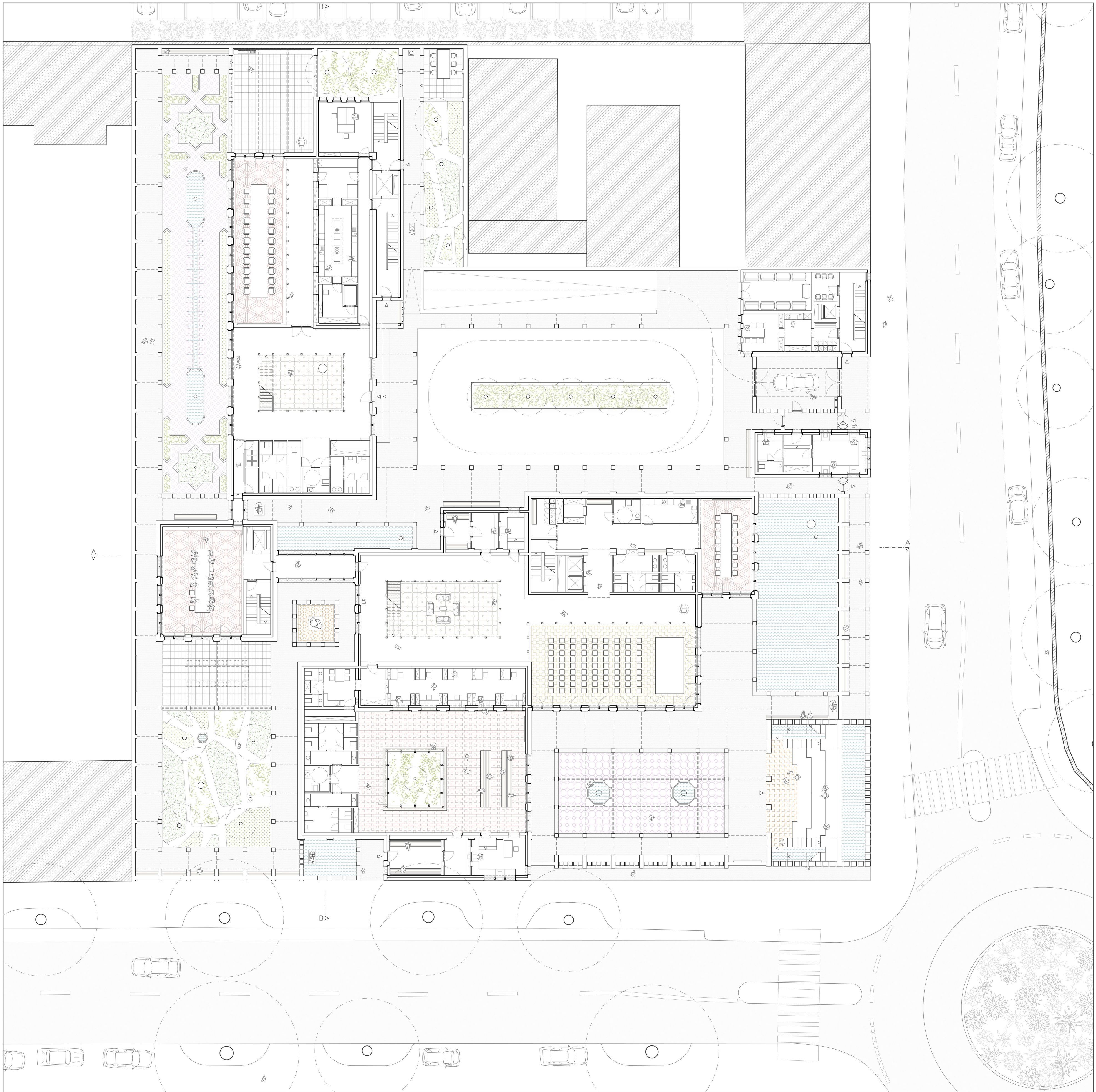
Grundriss Erdgeschoss M 1_200
