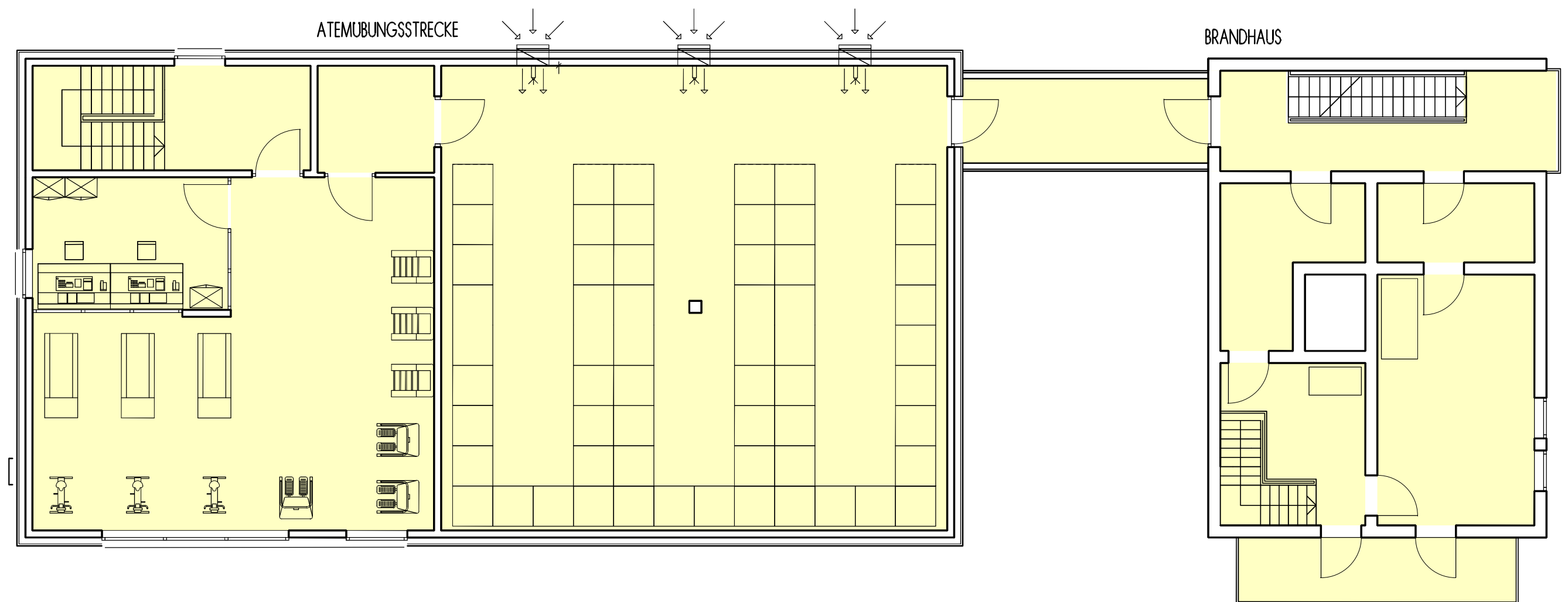
GRUNDRISS EBENE +1
