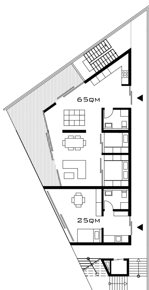
FLOORPLAN ALTERNATIVE
