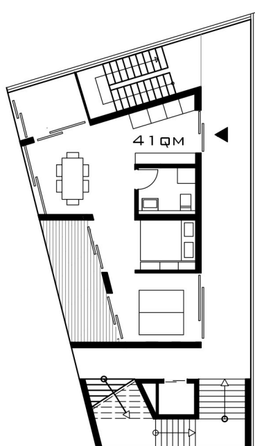
FLOORPLAN 1.FLOOR
