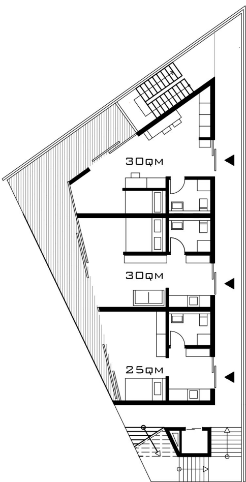
FLOORPLAN 1.FLOOR
