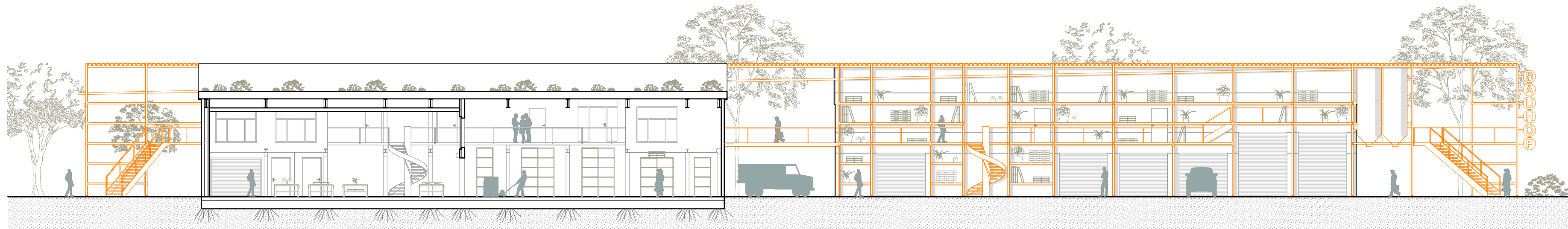
Section + Elevation North | 1:200 | C-C
