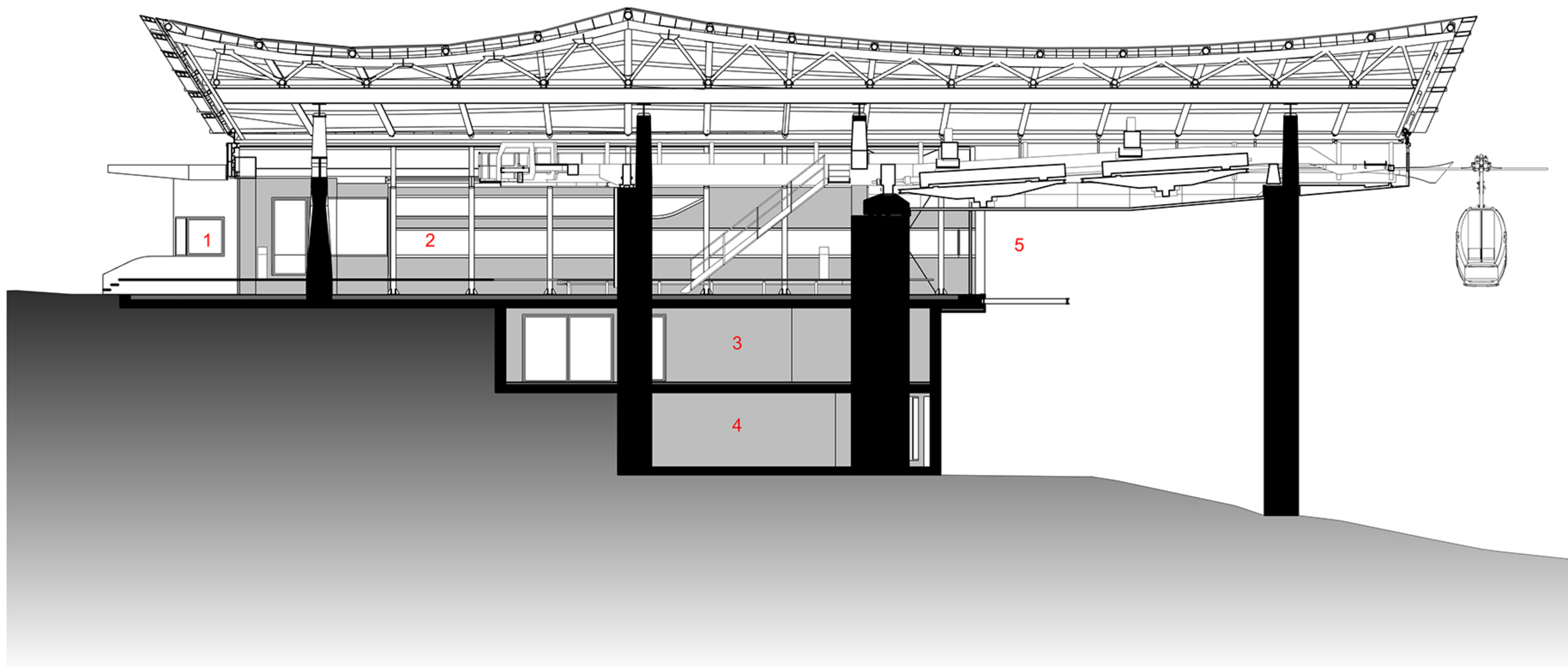
HILL STATION LONGITUDINAL SECTION
