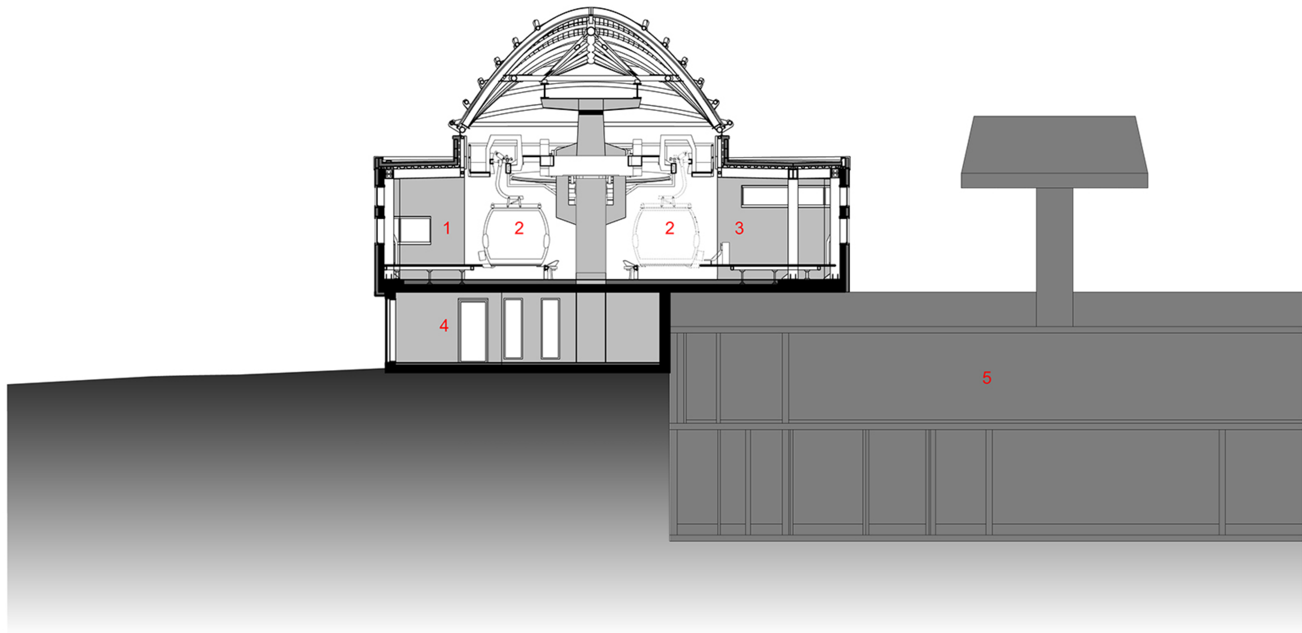
HILL STATION CROSS SECTION
