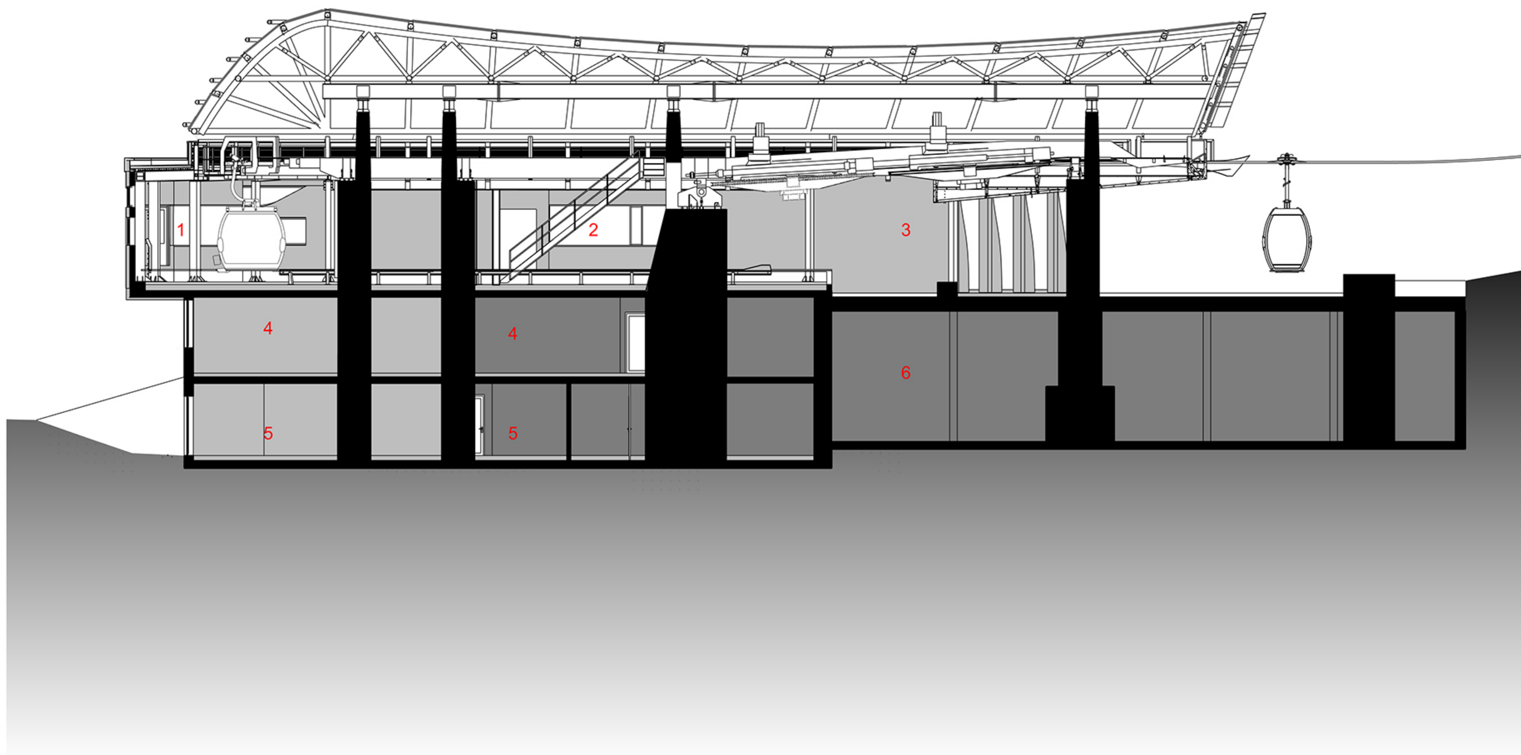
VALLEY STATION LONGITUDINAL SECTION
