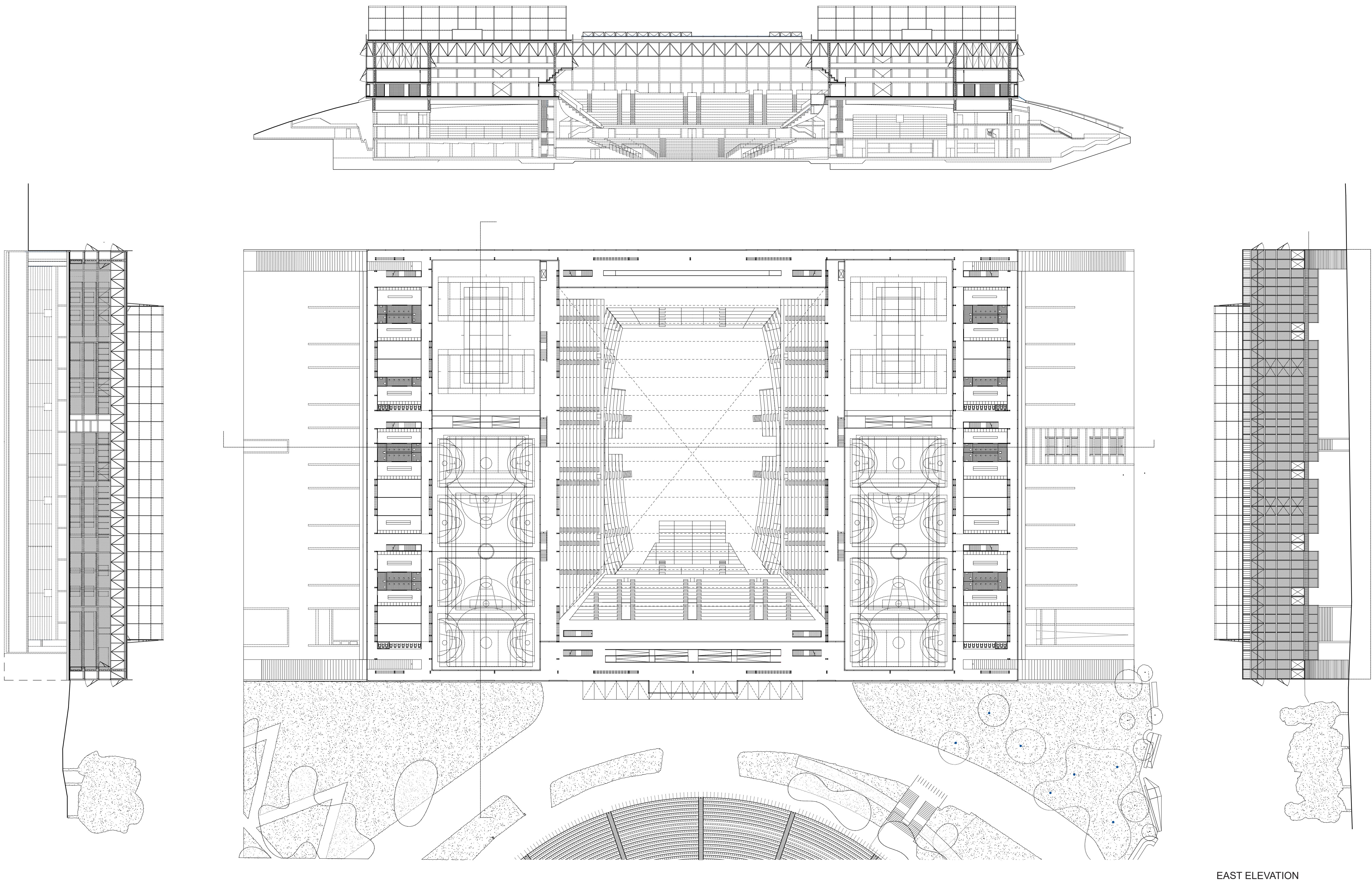
EAST ELEVATION
