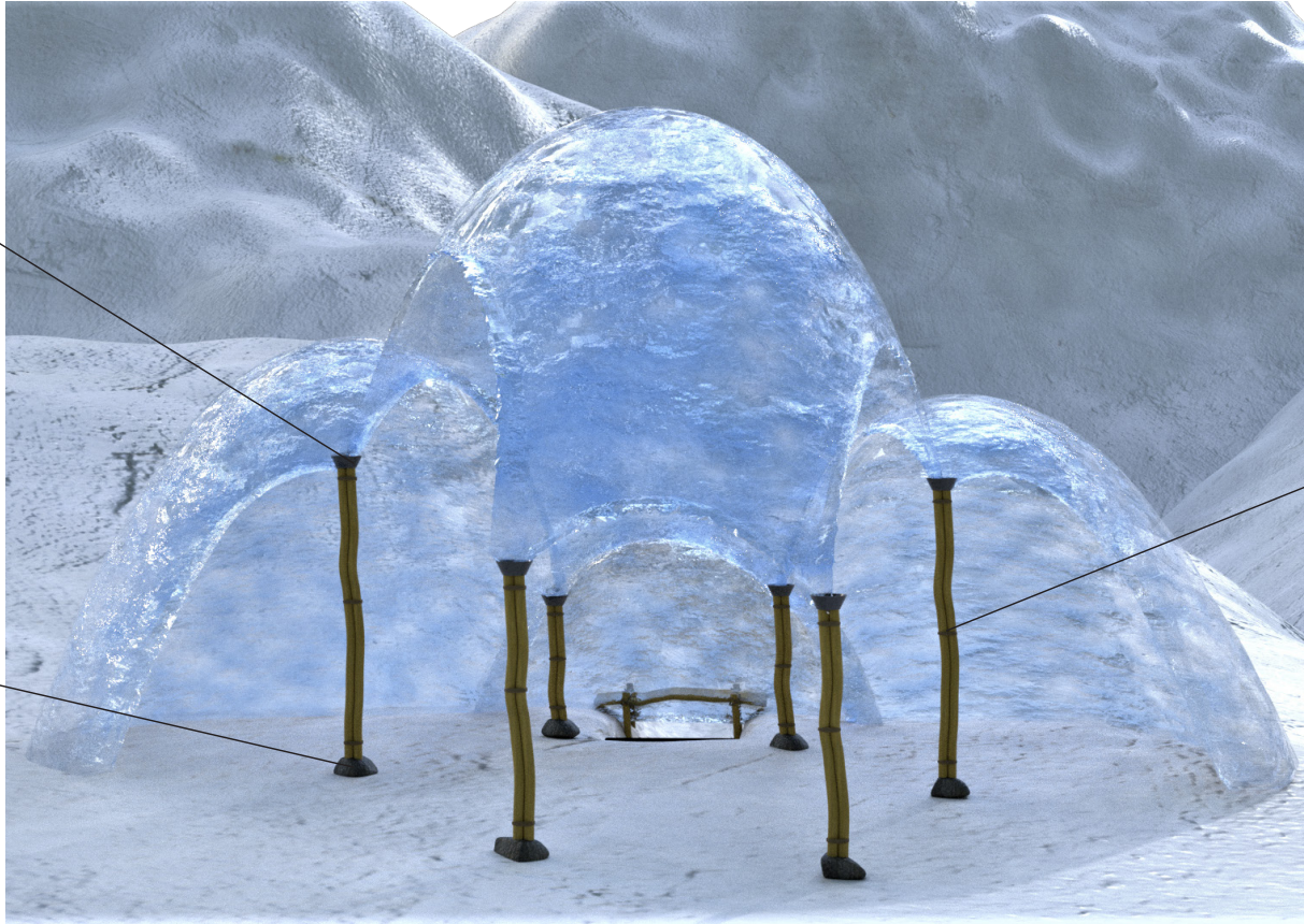
connection between Ice shells and bamboo columns via metal hopper plugged into the bamboo canes
