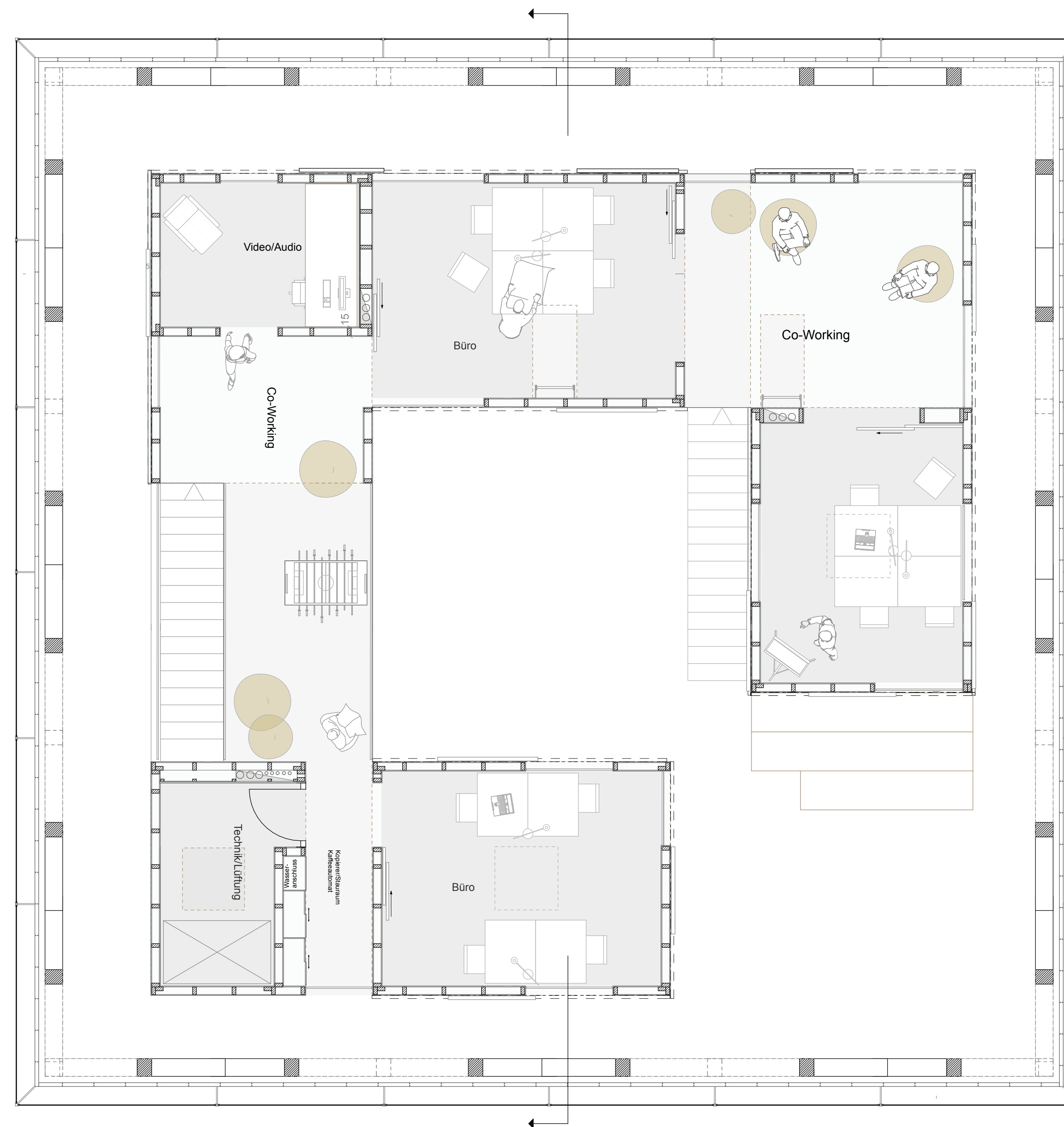
Floorplan upper level
