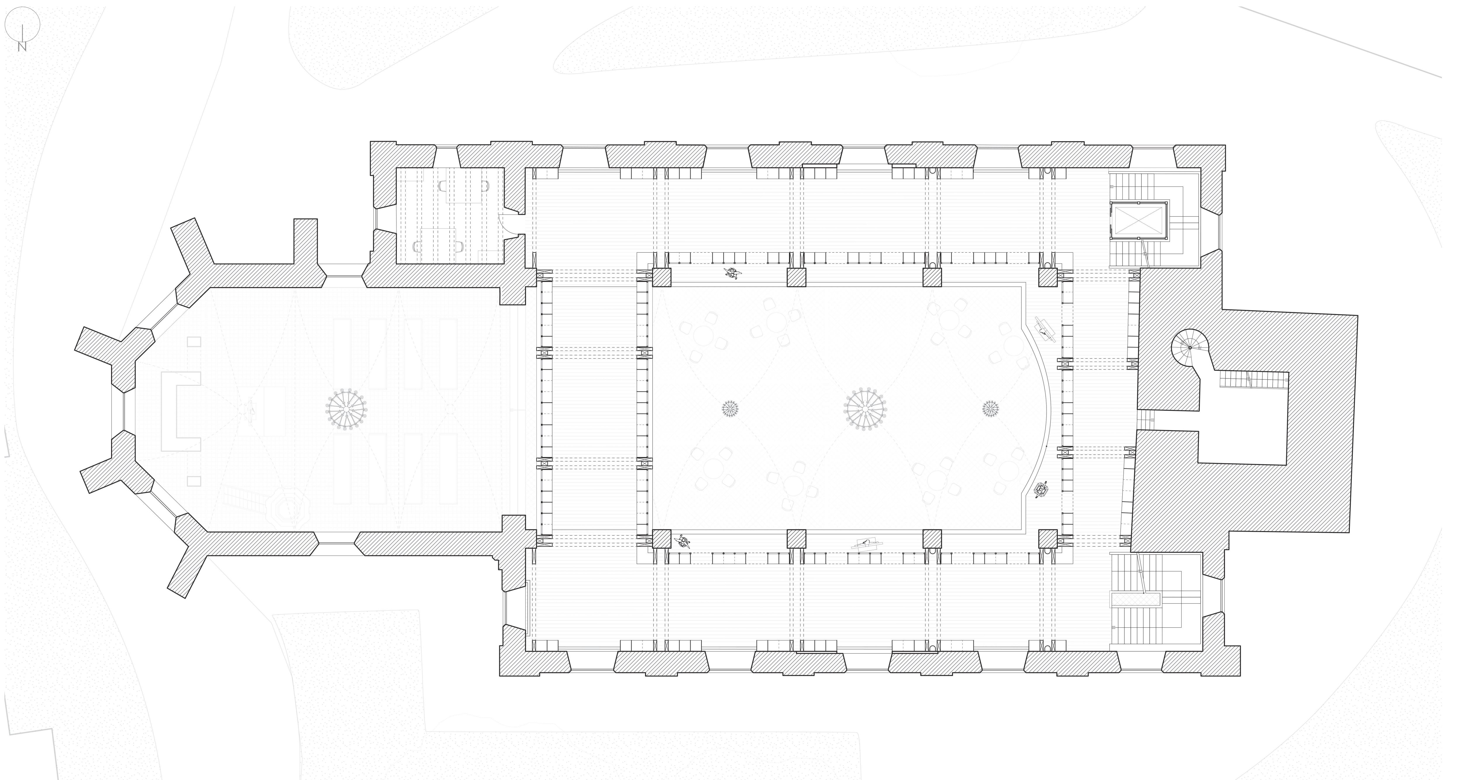
Grundriss 1. Empore M1:100
