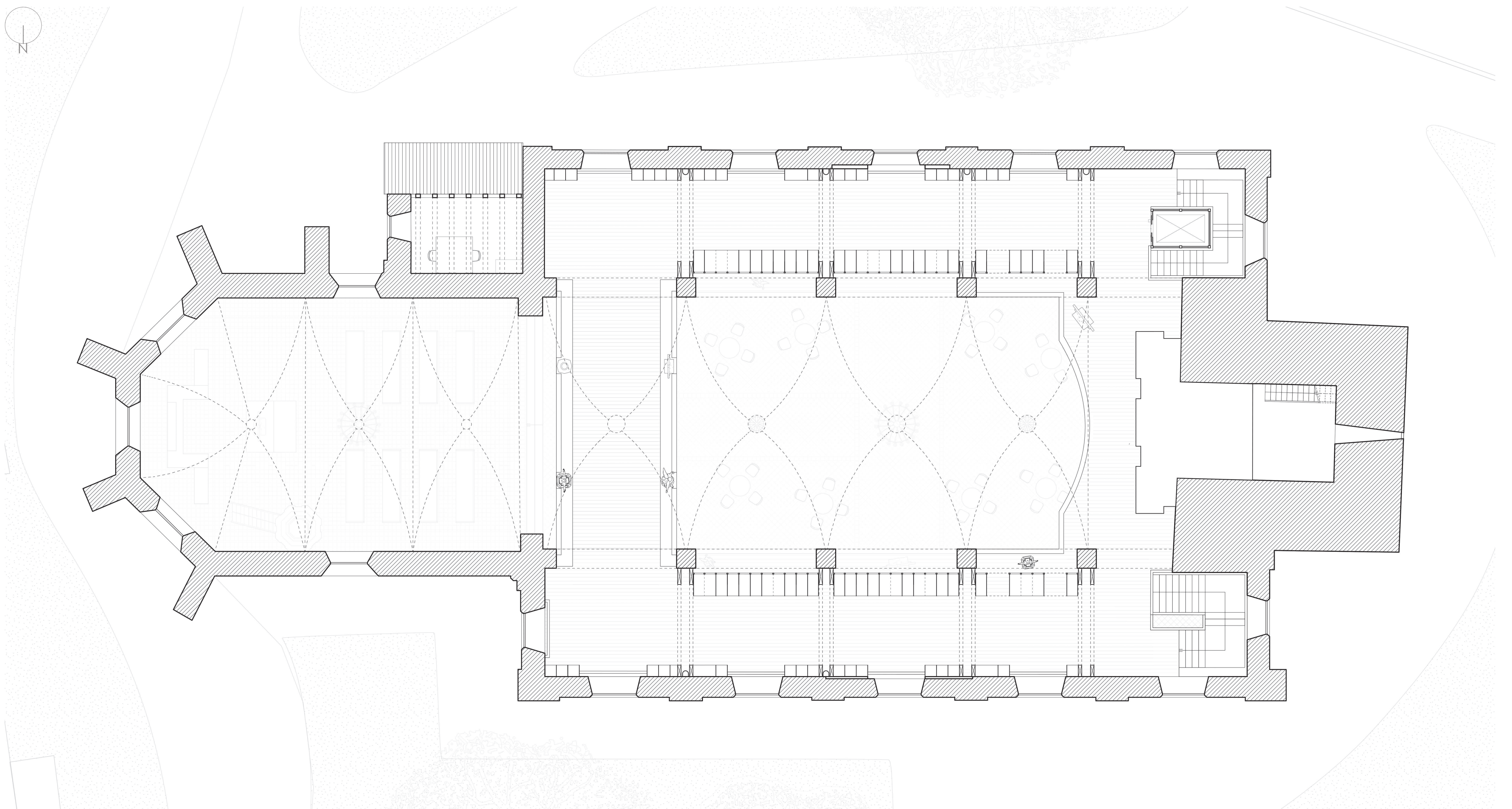
Grundriss 2. Empore M1:100
