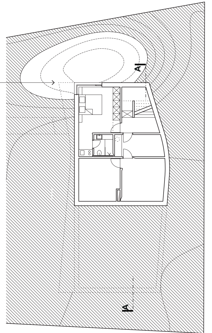
Basement 1:200
