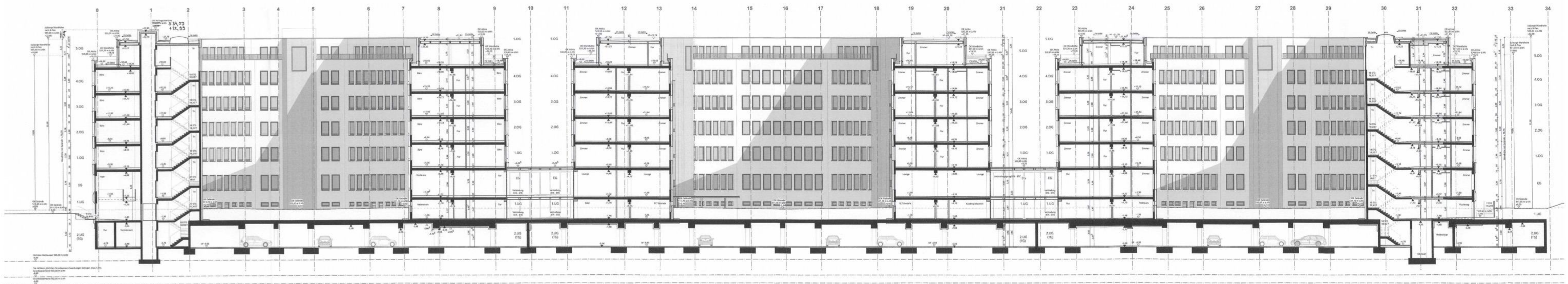
Schnitt S1 - S1 (BTX), M 1:200
