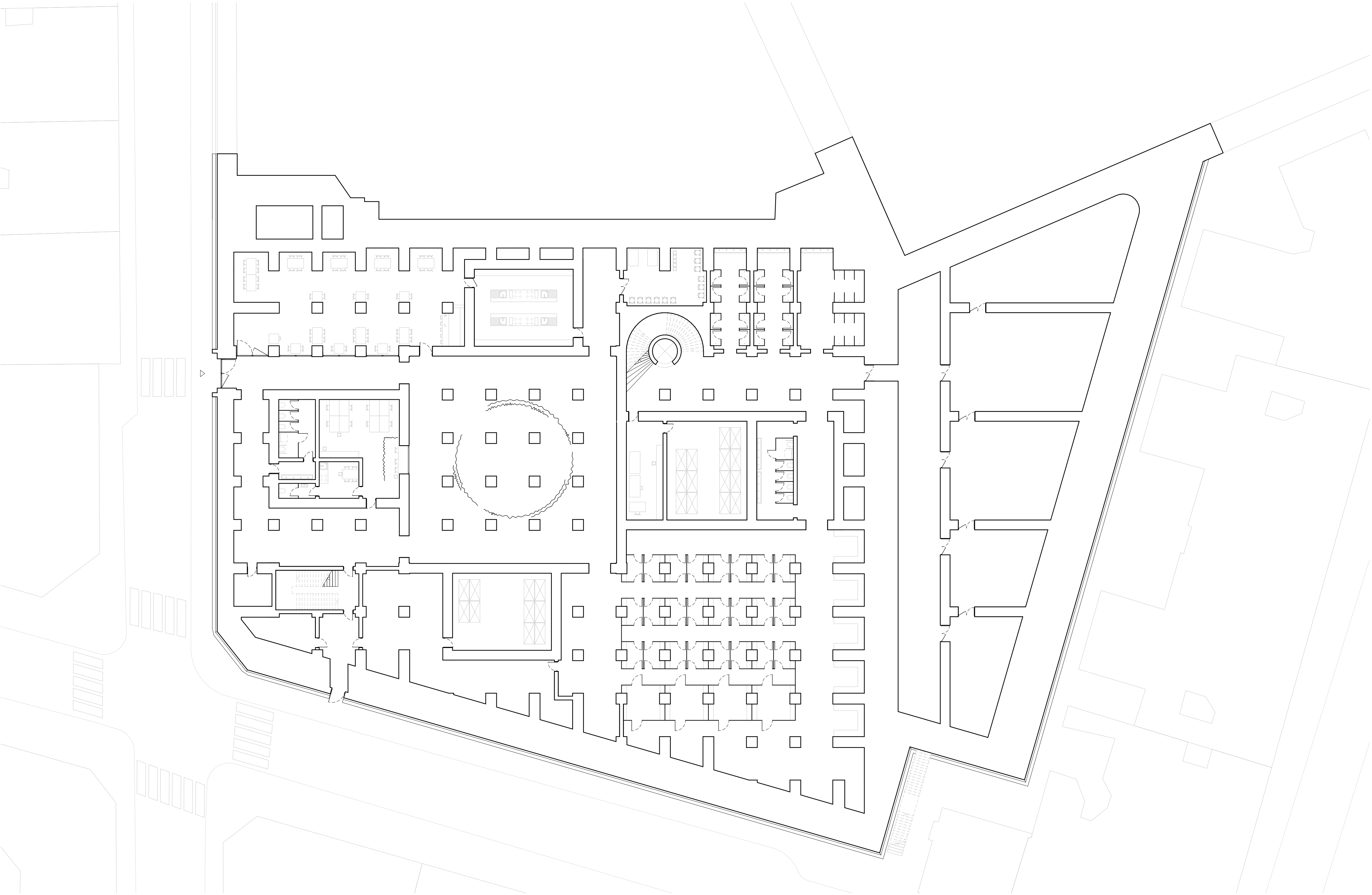
Erdgeschoss 1_200
