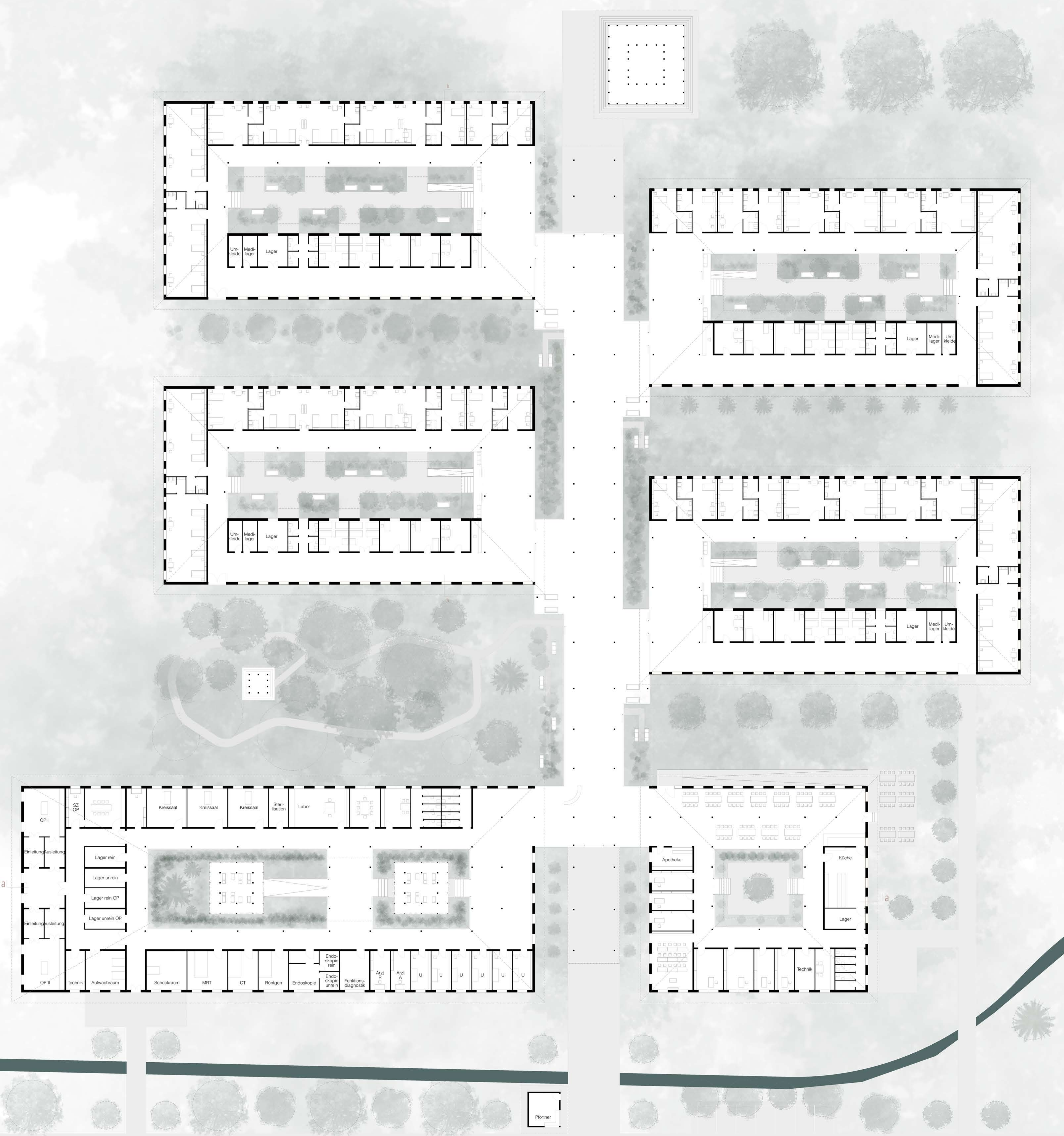
GRUNDRISS_EG, M 1:200
