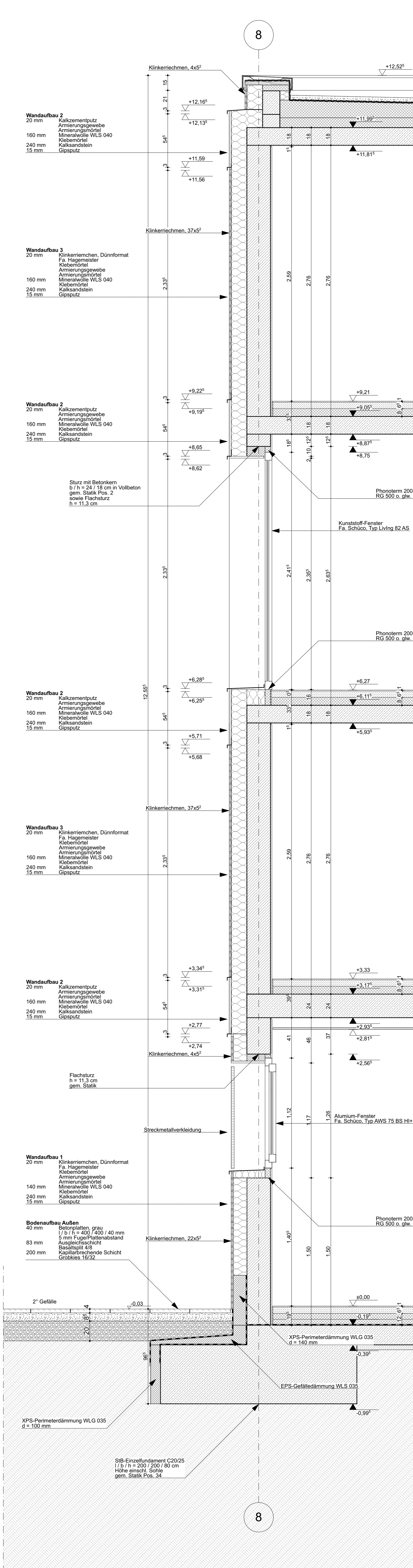
REGELFASADE | SERVICE
