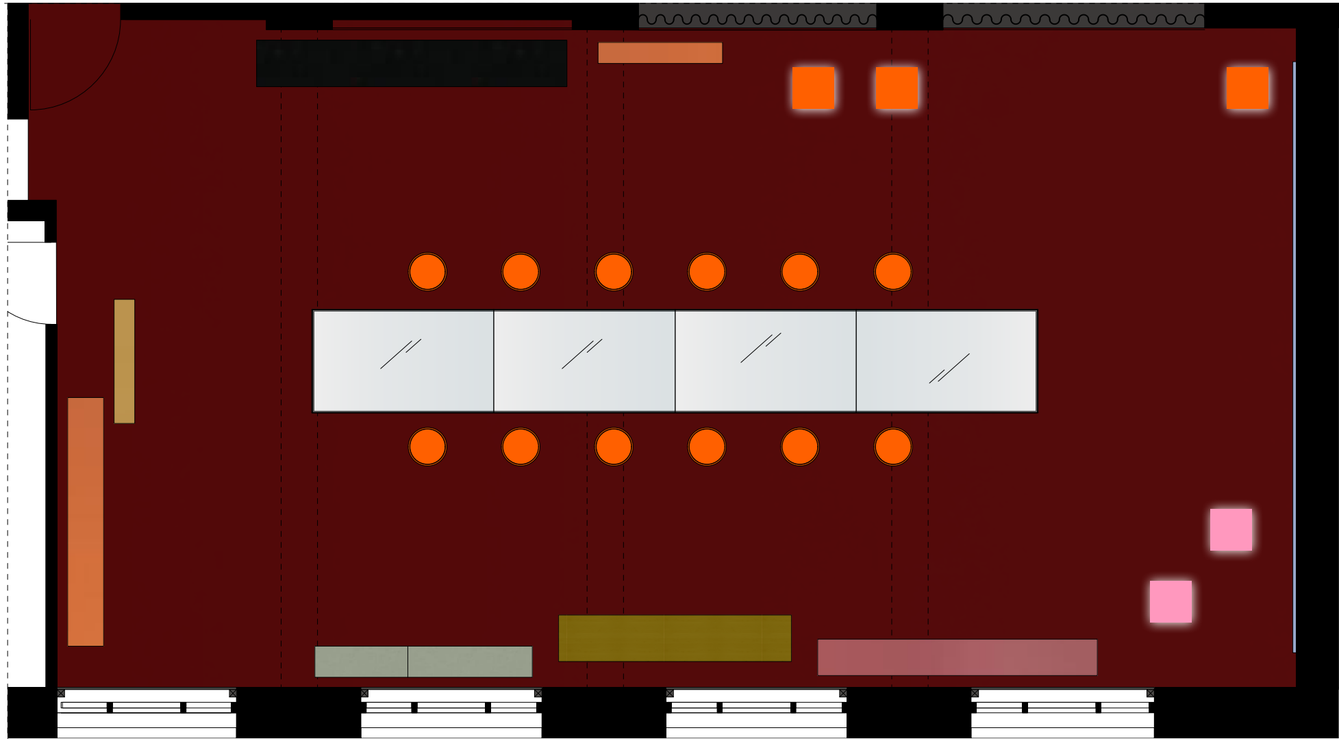
GRUNDRISS M 1: 50
