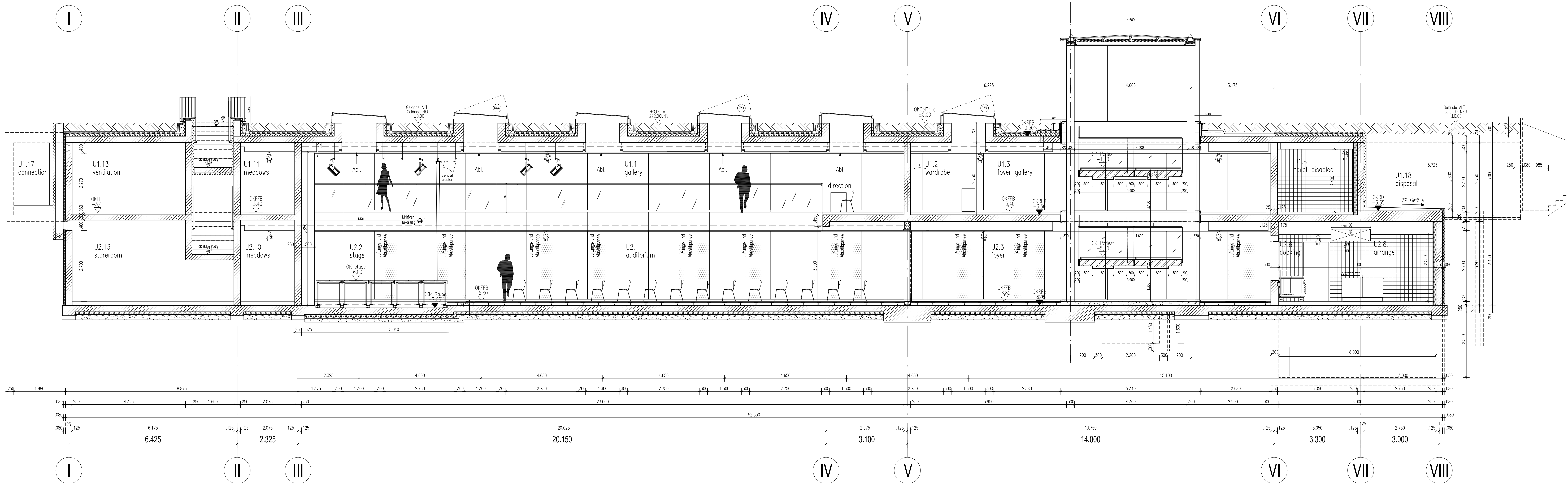
section 1-1
