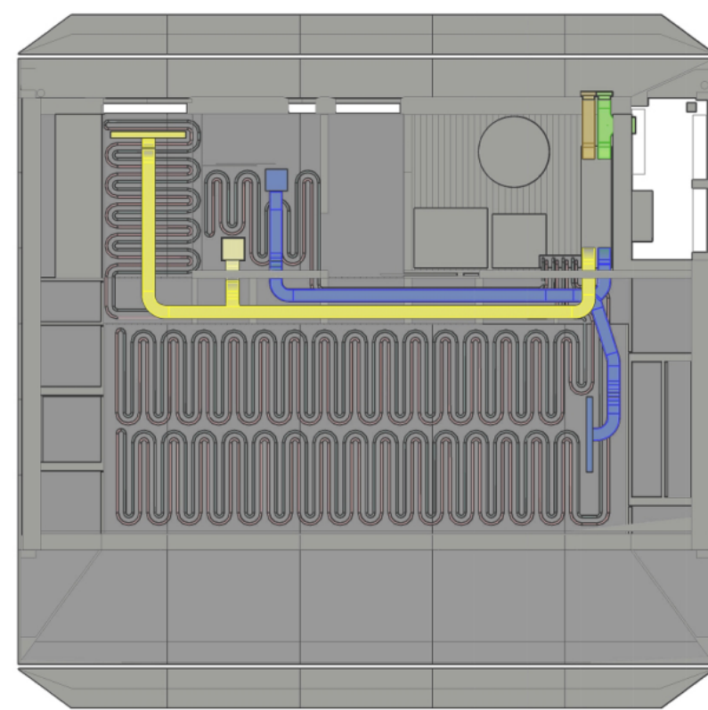
HEIZ-/KÜHLDECKE
