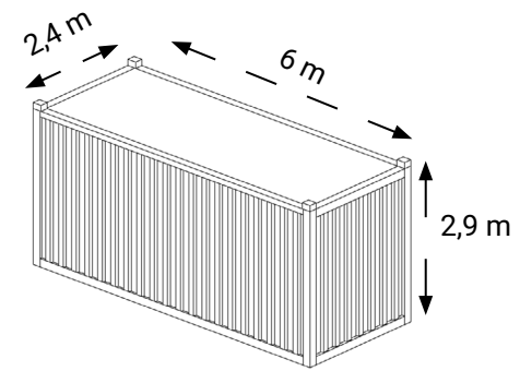
20 ft Offshore Container Standard
