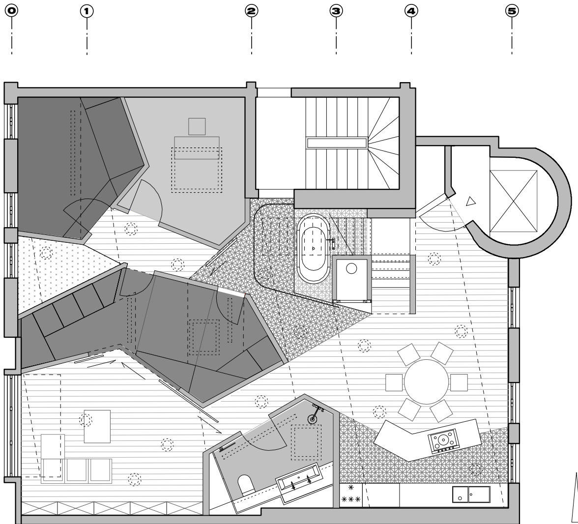
floorplan 1:100
