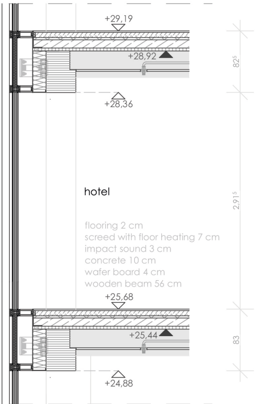
vertical section scale 1:20
