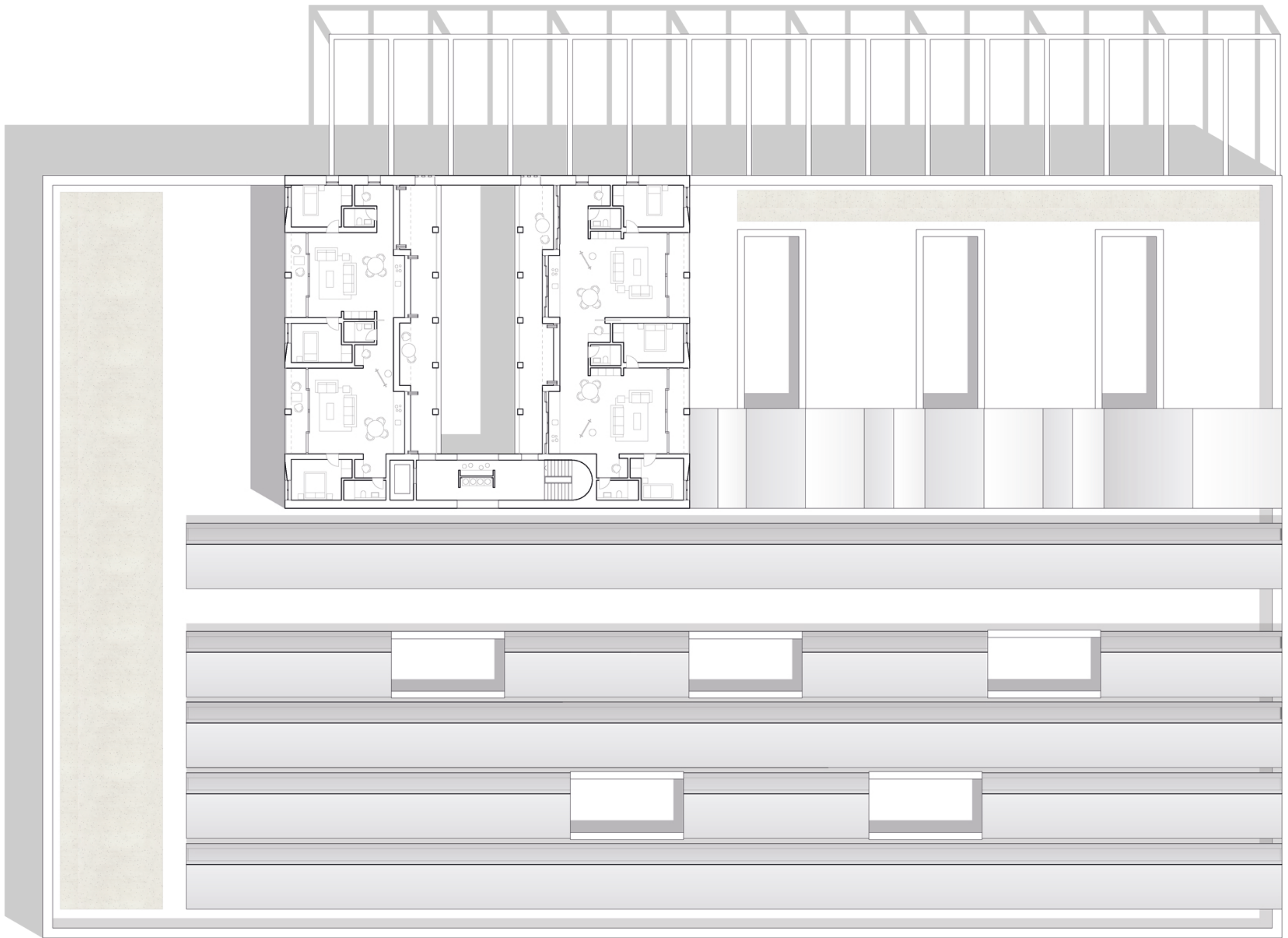
Grundriss 3OG M 1:200
