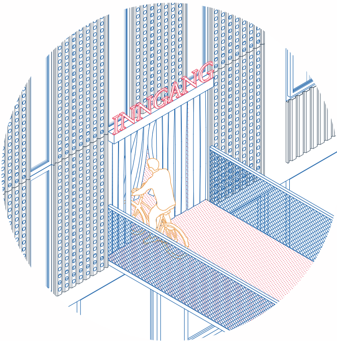
axonometry façade public 1:50
