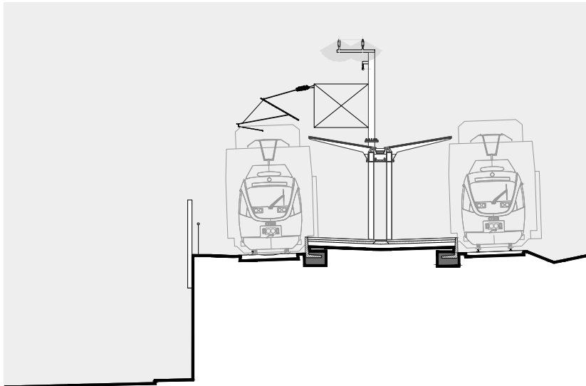
Section 1-1
