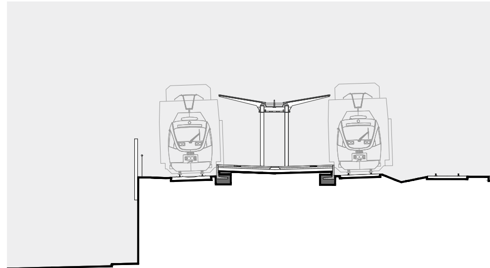
Section 2-2
