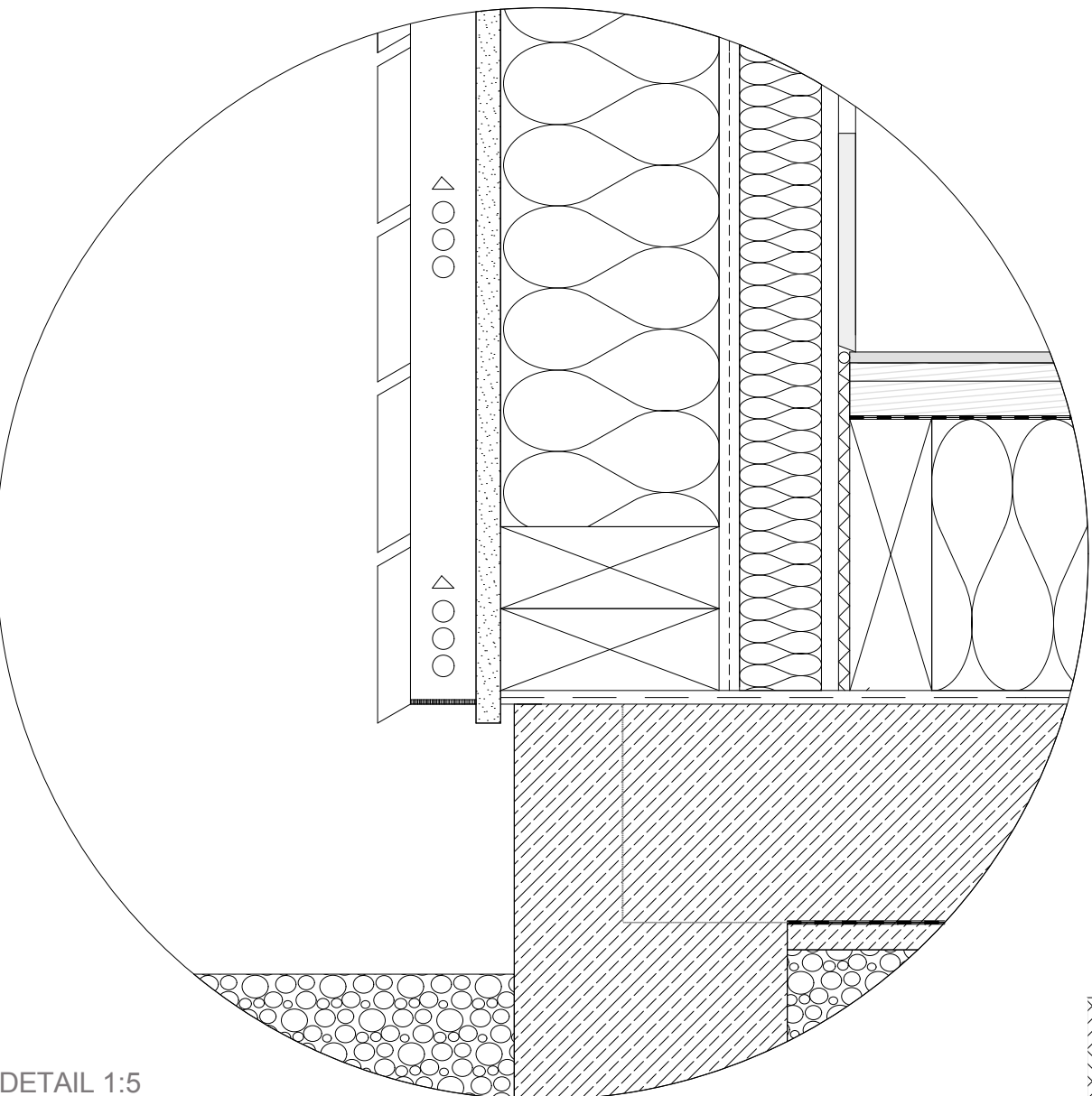
DETAIL 1:5
