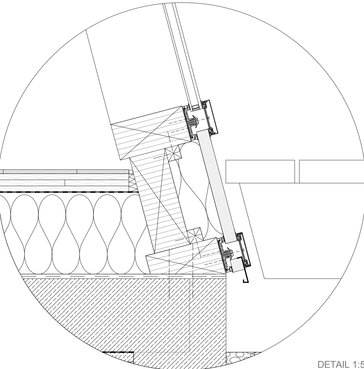
DETAIL 1:5
