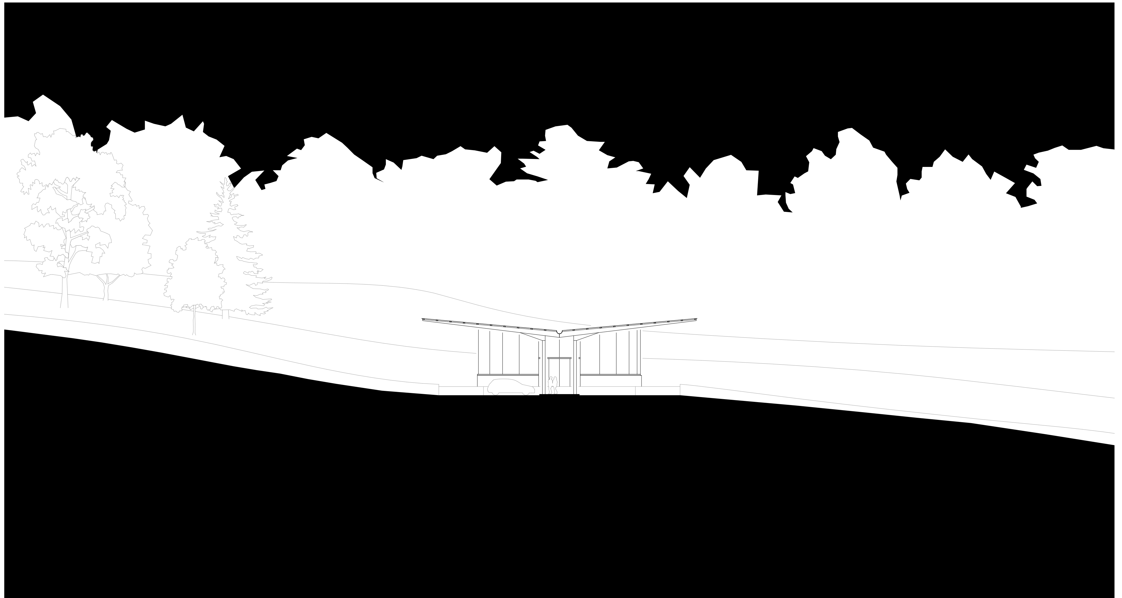
Schnitt Ost-West
