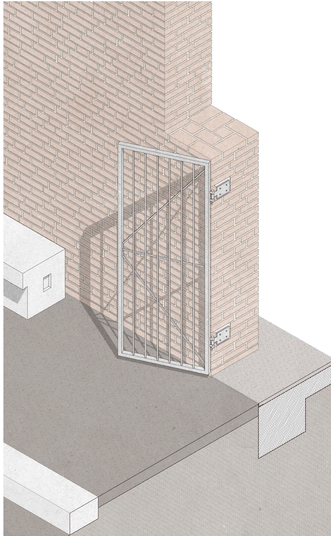
a galvanized steel gate and its wall mount
