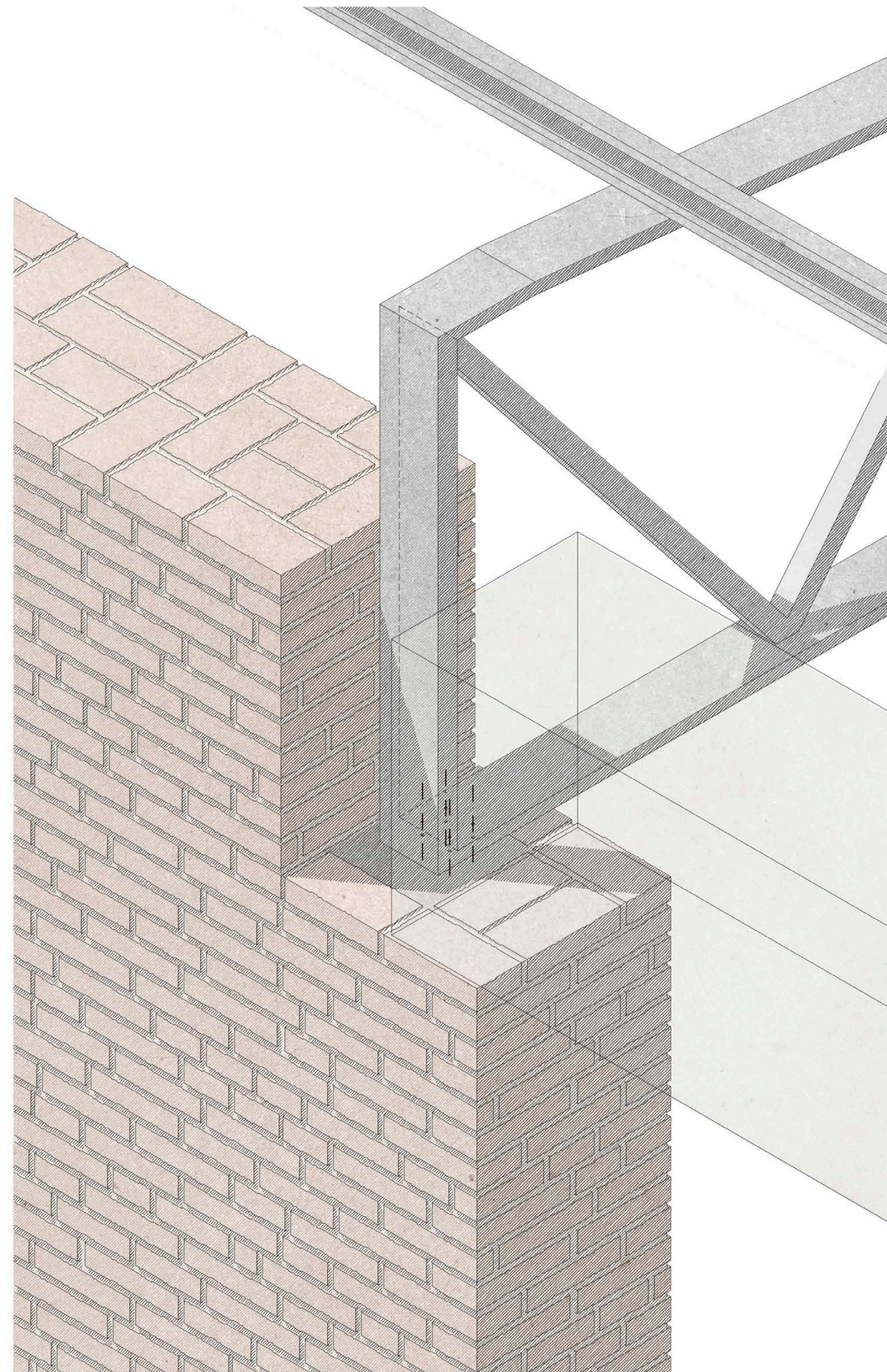
a truss-wall junction detail
