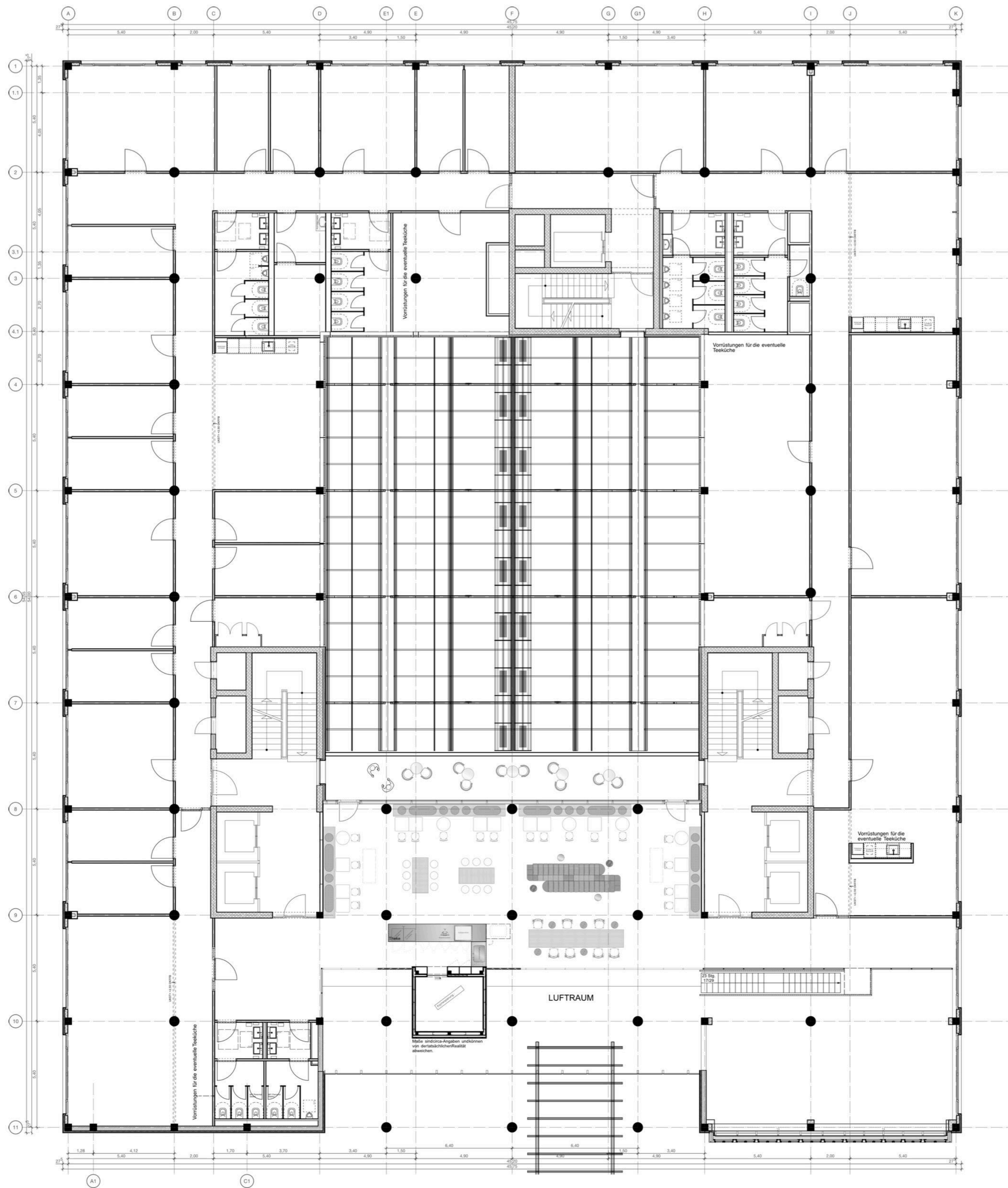
GRUNDRISS 1.OG | INFORMAL MEETING
