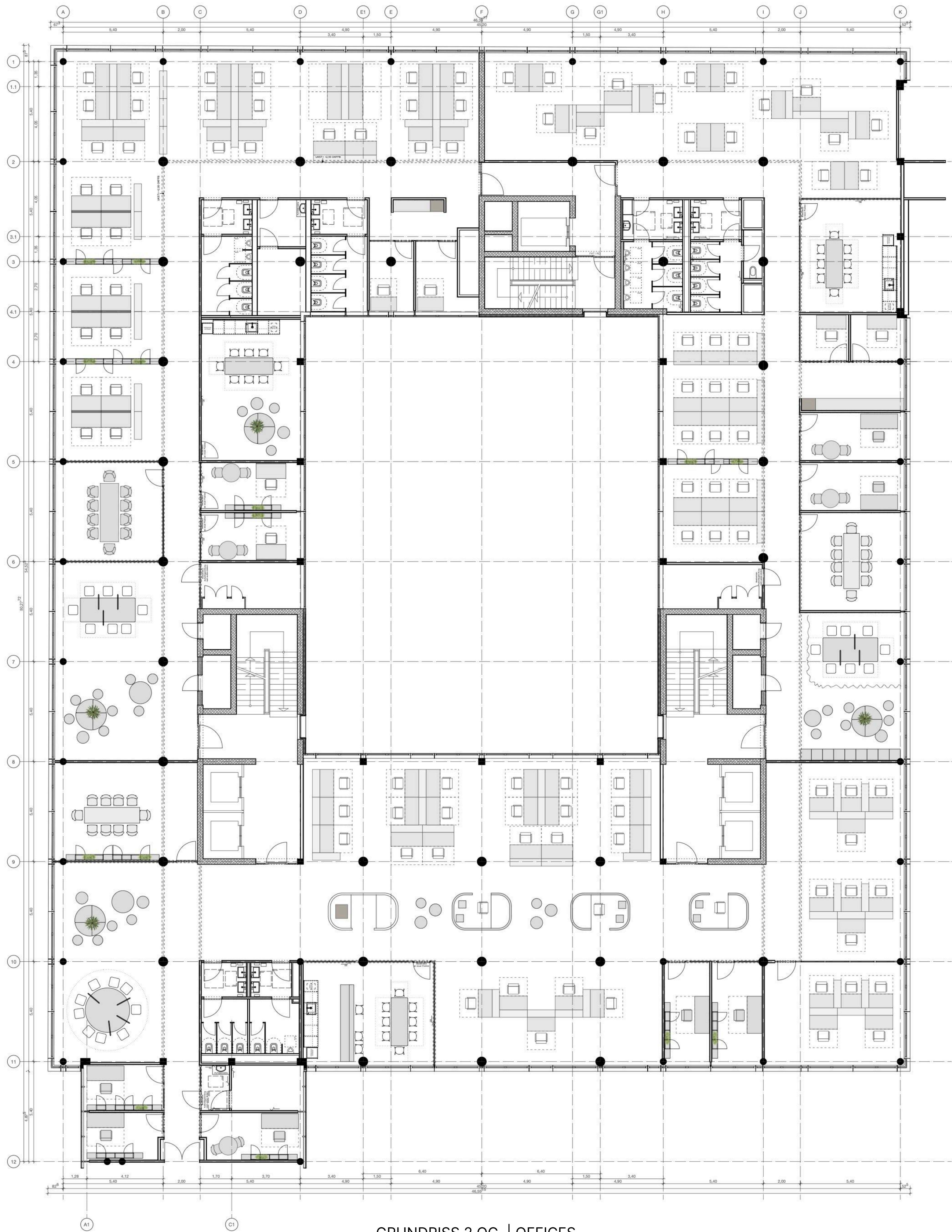
GRUNDRISS 2.OG | OFFICES
