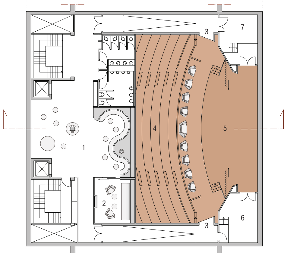
Floor Plans
