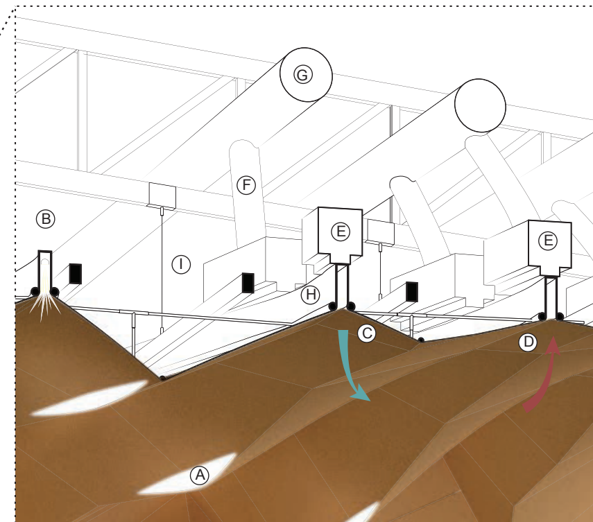
Detail
