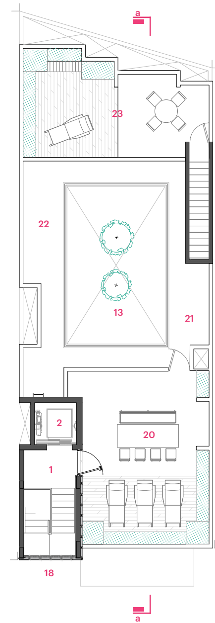
roof plan
