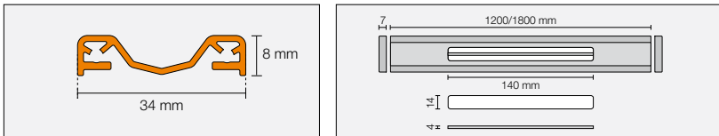
Schlüter®-KERDI-LINE-VARIO-COVE 34 A
