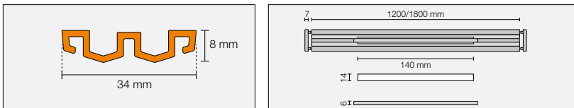
Schlüter®-KERDI-LINE-VARIO-WAVE 34 A
