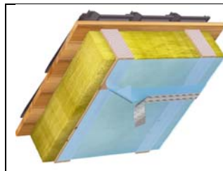
Abb. 4: Überlappung innen
